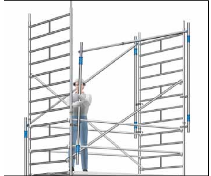
Fig. 5: Upward movement of the advance guardrail system
