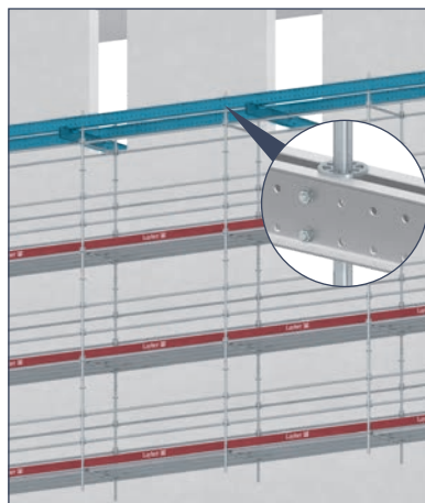
Suspended bracket scaffolding
