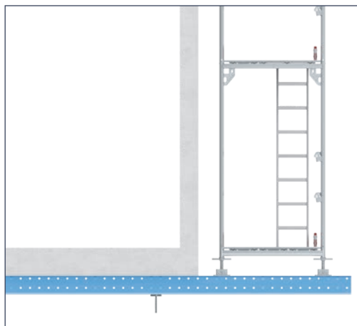
Bracket scaffolding anchored to the slab
