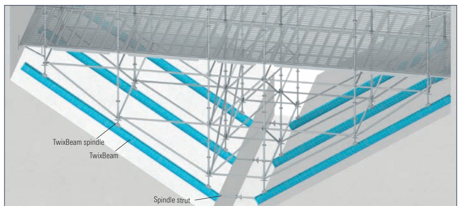
Beam structure for adjustment to funnel-like boiler
