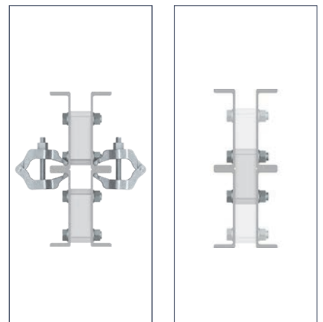
Beams placed one above the other secured using beam clamps (left) or with the spacer (right)
